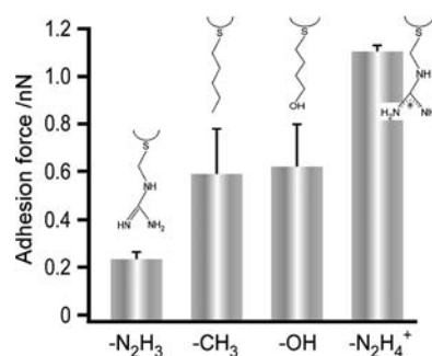
Figure 3. AFM adhesion force between Au-coated AFM tips modified with a layer of organothiols and the silicalite-1 (010) surface. The thiol terminal groups mimic ZGM moieties. A pH 12 solution was used for -OH and -CH_3 tips, and pH 11 ( -N_2H_4^+ ) and pH 13 ( -N_2H_3 ) were used for amidinium tips. Each force is an average from 8000 pull-off curves on multiple crystals (error bars equal one standard deviation).
