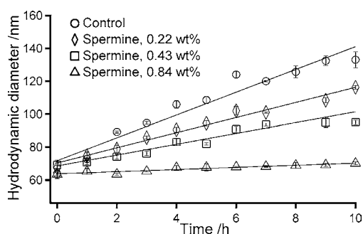
Figure 5. DLS seeded growth experiments measuring the temporal change in the hydrodynamic diameter of silicalite-1 seeds suspended in a silica growth solution at 85\text{ }^\circ\text{C} . The growth rate (slope) decreases linearly with increasing spermine concentration. Experimental data (symbols) are an average of four measurements and error bars equal two standard deviations. Lines are linear regression.
