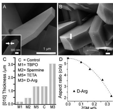
Figure 4. Effect of modifiers on silicalite-1 crystal morphology. SEM images reveal crystals synthesized with < 0.5\text{ wt\%} spermine (A) and D-Arg (B) have decreased and increased thickness, respectively. C) ZGMs selectively tailor the thickness of silicalite-1 platelets along the b -axis (i.e. diffusion length in less tortuous [010] channels). D) D-Arg preferentially binds to (302) faces, causing a monotonic reduction in the c/a (length/width) aspect ratio of basal (010) faces with increasing D-Arg wt%.
